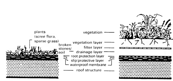
⑦ Retrospective roof cultivation at low expense
